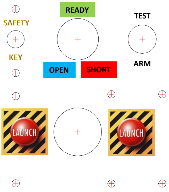
HANDHELD SMART LAUNCH CONTROLLER
